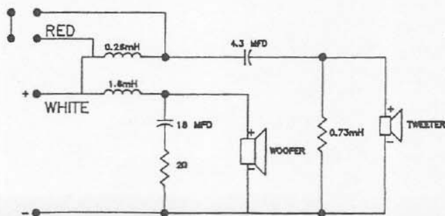
CROSSOVER SCHEMATIC
